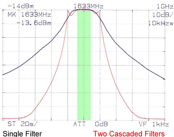
S21 3-Pole Interdigital Filter 1600 - 1670 MHz
