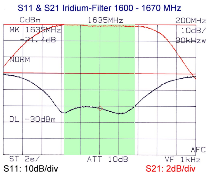
S21 3-Pole Interdigital Filter 1600 - 1670 MHz
