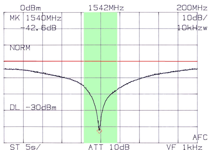
S11 Inmarsat-Antenna 1525 - 1559 MHz
